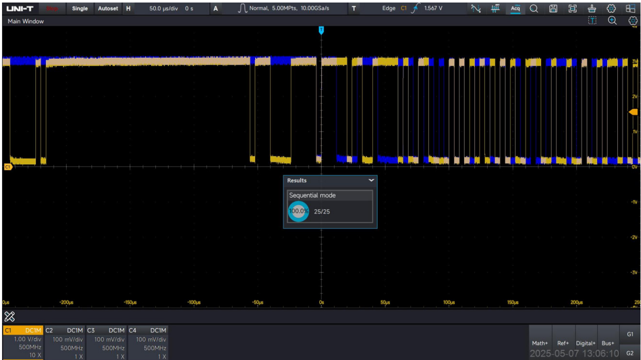
By leveraging the high capture efficiency of Sequential mode, 25 complete CAN protocol frames were successfully captured for comparison. Analysis revealed timing errors in the transmitted bits. In the figure, the blue waveform represents the reference frame. Dark yellow segments indicate matching portions, while yellow segments highlight deviations.
